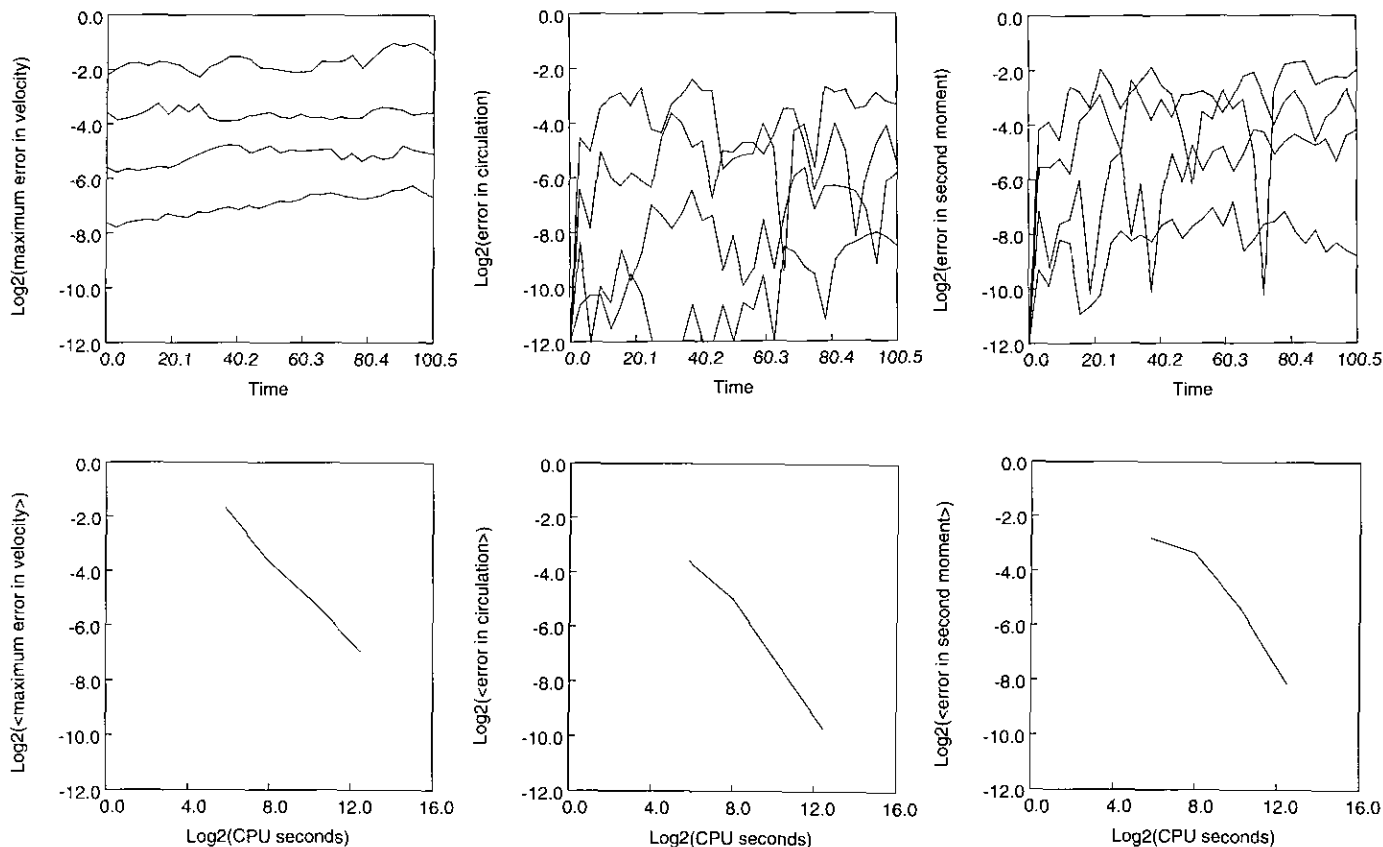
FIG. 15. Comparison with vortex-blob methods; relative L^\infty velocity, circulation, and moment errors (left to right) versus time (first row) and the corresponding time-averaged errors versus SPARC-2 CPU time (second row) for our method. The four runs plotted used the following parameters: mesh sizes h = 0.4, 0.2, 0.2, \text{ and } 0.1 ; N = 29, 113, 441, \text{ and } 1793 vertices; n = 64, 96, 128, \text{ and } 192 time steps.
