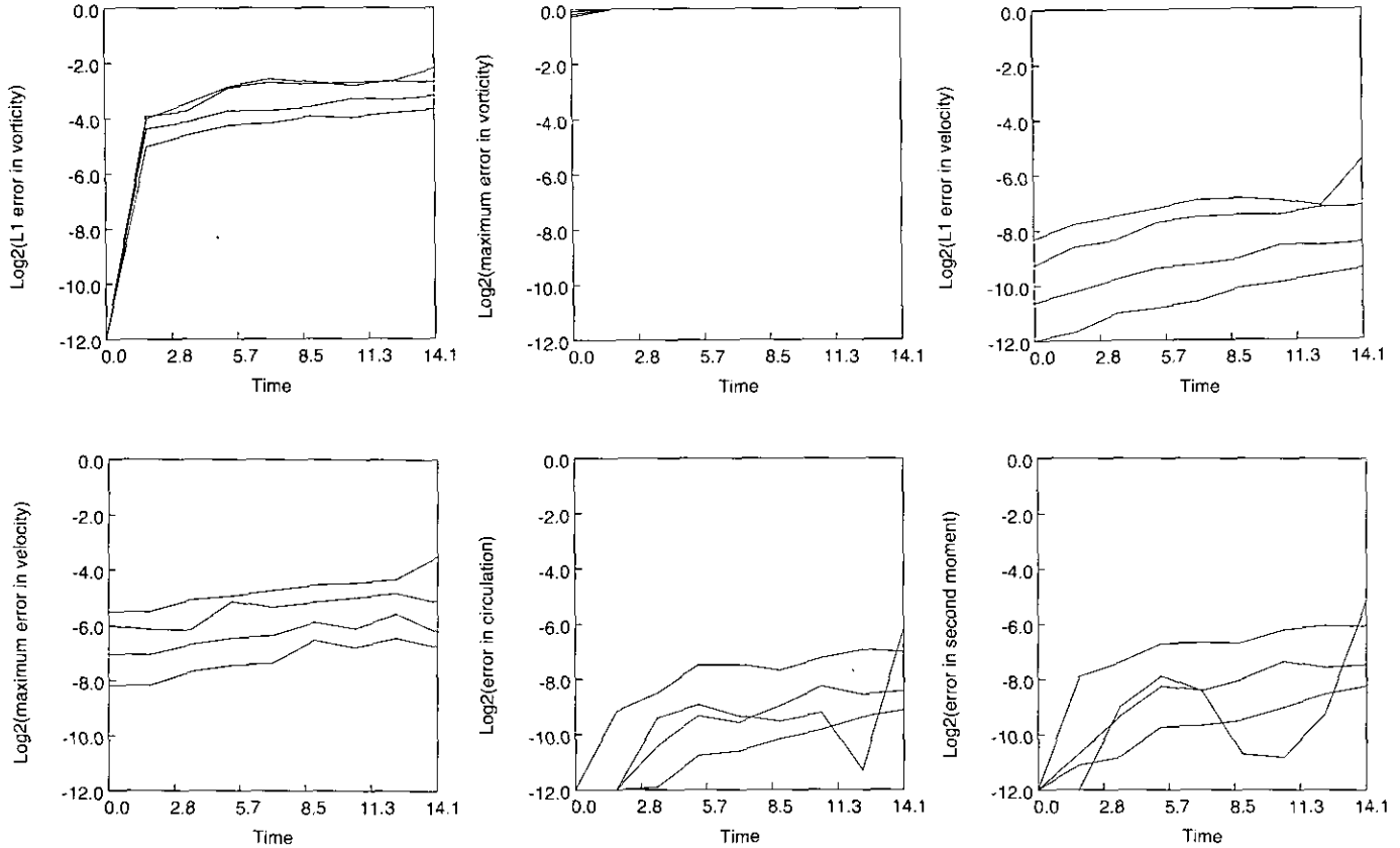
FIG. 22. Errors for the Kirchhoff elliptical vortex. First row: Relative L^1 and L^\infty errors in vorticity and L^1 error in velocity versus time. Second row: Relative L^\infty error in velocity, circulation, and second moment errors versus time. The four runs plotted used the following parameters: mesh tolerances \epsilon = 0.064, 0.016, 0.004, and 0.001 ; N = 468, 1064, 2320, and 4700 vertices; n = 32, 48, 64, and 96 time steps.
