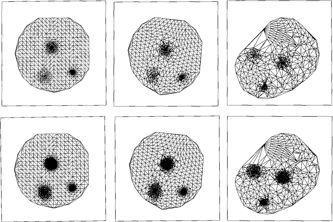
FIG. 23. Three interacting patches of smooth vorticity, at times t = 0, 25 , and 200 (left to right), with \epsilon = 0.016 (top row) and 0.004 (second row).
