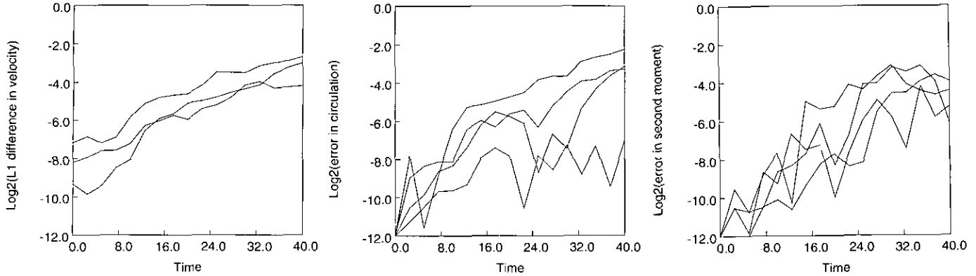
FIG. 26. Errors for constant patches of vorticity, estimated by differencing. Relative L^1 error in velocity, circulation errors, and second moment errors vs time.
