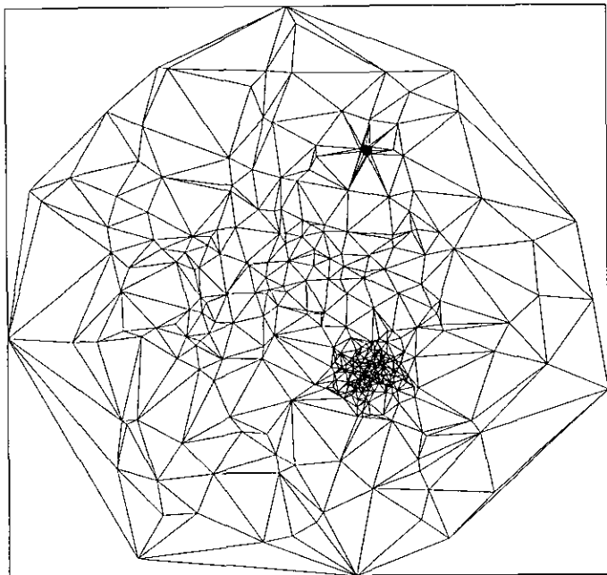
FIG. 10. Sample Delaunay triangulation of N = 800 nonuniform points.
