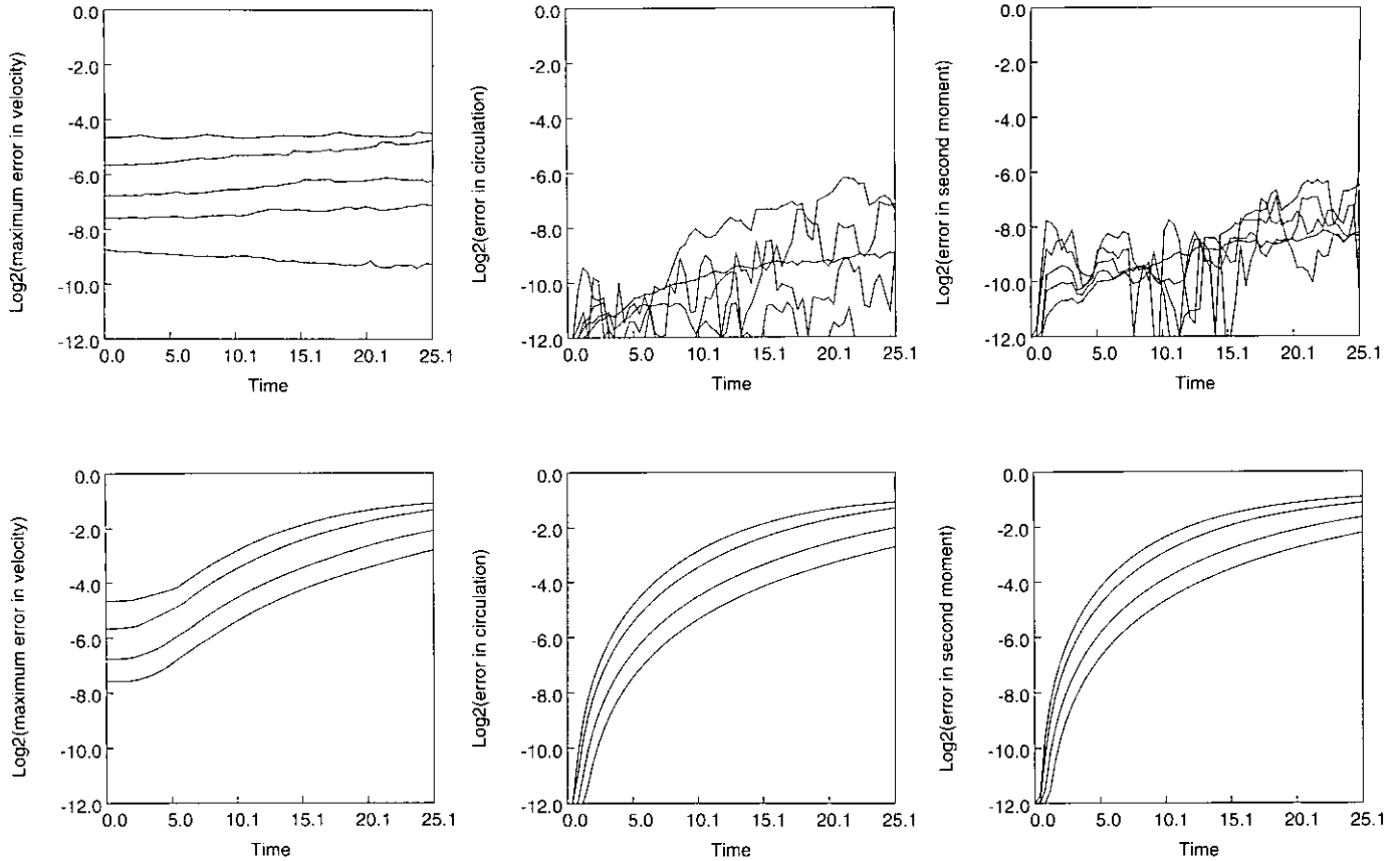
FIG. 17. Comparison between fixed topology and Delaunay triangulation with h = \frac{1}{8}, \frac{1}{12}, \frac{1}{16}, \frac{1}{24} . First row: Relative L^\infty error in velocity, circulation errors and second moment errors versus time for Delaunay triangulation. Second row: the same quantities for fixed topology.
