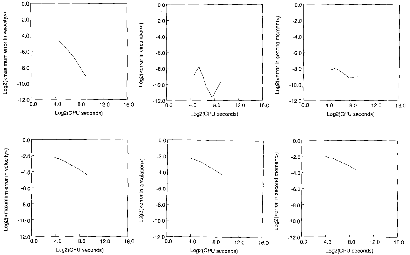
FIG. 18. Comparison between fixed topology and Delaunay triangulation with h = \frac{1}{6}, \frac{1}{8}, \frac{1}{12}, \frac{1}{16}, \frac{1}{24} . First row: Time-averaged relative L^\infty error in velocity, circulation errors and second moment errors versus Cray-2 CPU time for Delaunay triangulation. Second row: the same quantities for fixed topology.
