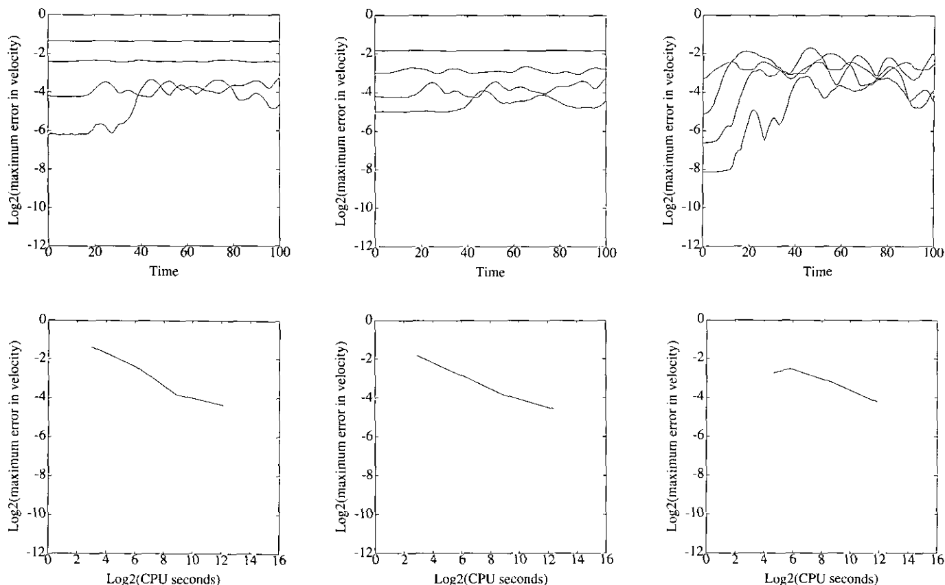
FIG. 14. Errors versus time for the vortex blob method with h = 0.4, 0.2, 0.1, and 0.05 and \Delta t = 0.05 . Top row: Relative L^\infty errors in velocity versus time. Second row: Time-averaged relative L^\infty errors in velocity versus SPARC-2 CPU time in seconds. Left column: Supergaussian blob, q = 0.7 . Center: Supergaussian blob, variable q = 0.9, 0.8, 0.7, and 0.6 . Right: Finite-core blob, q = 0.4 .
