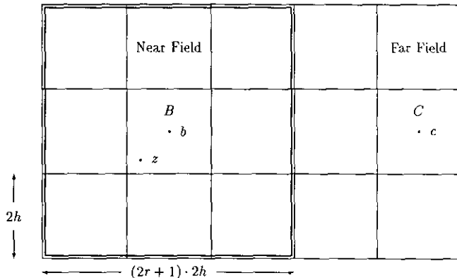
FIG. 11. Cells and centers for fast velocity evaluation, with r = 1 .
