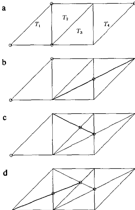
FIG. 13. An example of Mitchell's recursive newest-node bisection. Triangle T_1 is flagged for subdivision, but the peak (circle) of its neighbor T_2 does not lie opposite T_1 . Hence we must refine T_2 and its neighbor T_3 . Similarly, the peak of T_3 does not lie opposite T_2 , so we must refine T_4 and T_3 . The peak of T_4 lies opposite T_3 , so the recursion stops here. We then divide triangles backwards in pairs as shown in (b) through (d), until we have divided T_1 . The final triangulation is shown in (d).
