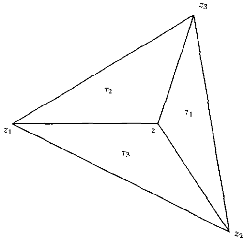
FIG. 1. Splitting up the computation of the Biot-Savart integral.
