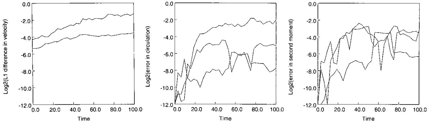
FIG. 24. Errors for smooth patches of vorticity, estimated by differencing. Relative L^1 error in velocity, circulation errors, and second moment errors vs time.
