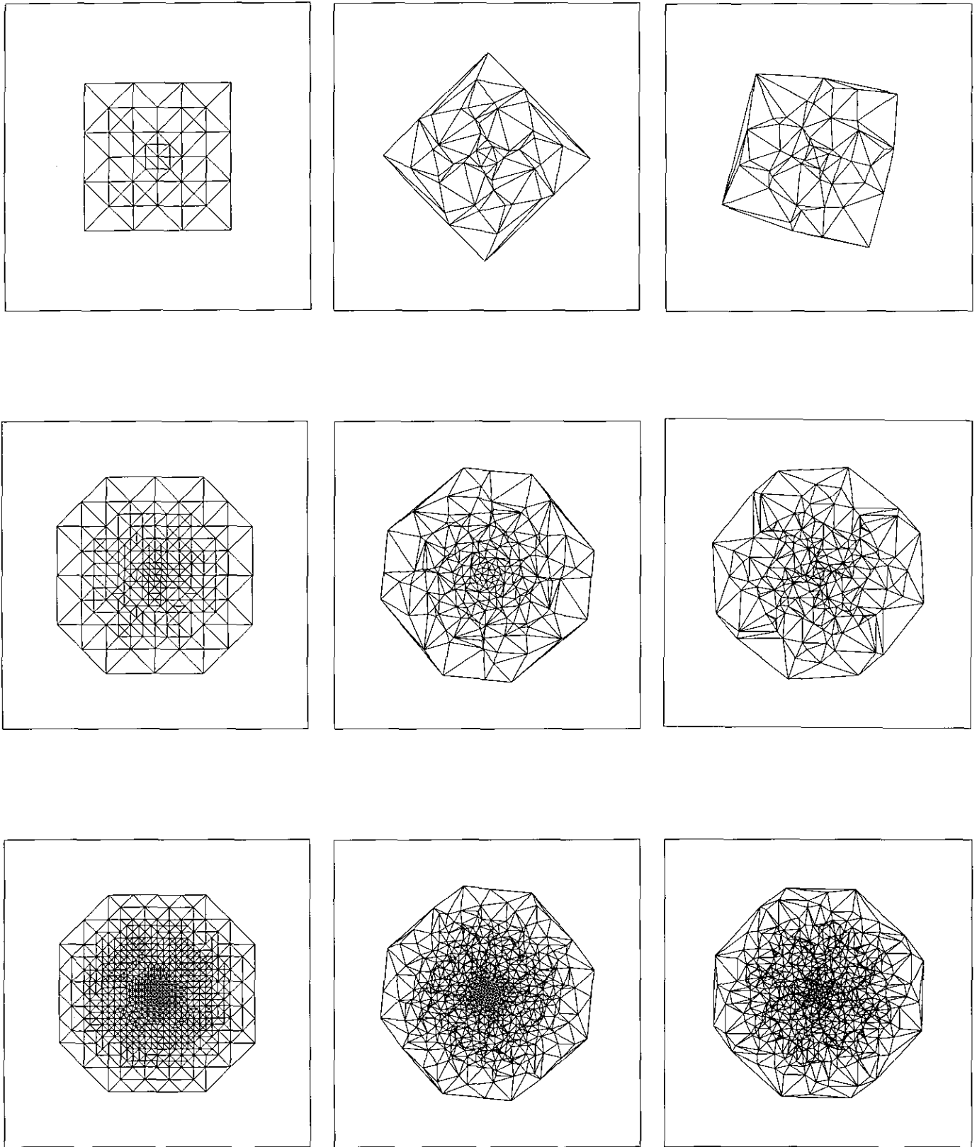
FIG. 19. Adaptive triangulation of Perlman's test case at times t = 0, 4\pi , and 32\pi (left to right), with \epsilon = 0.064 (top row), 0.016 (second row), and 0.004 (last row).
