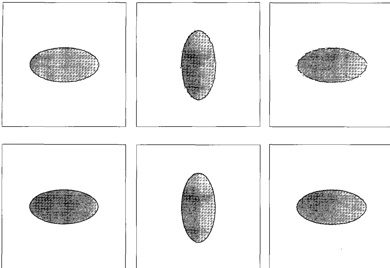
FIG. 21. Grayscale plots of the Kirchhoff elliptical vortex at times t = 0, T/4, and T/2 (left to right), with \varepsilon = 0.016 (top row) and 0.004 (last row).
