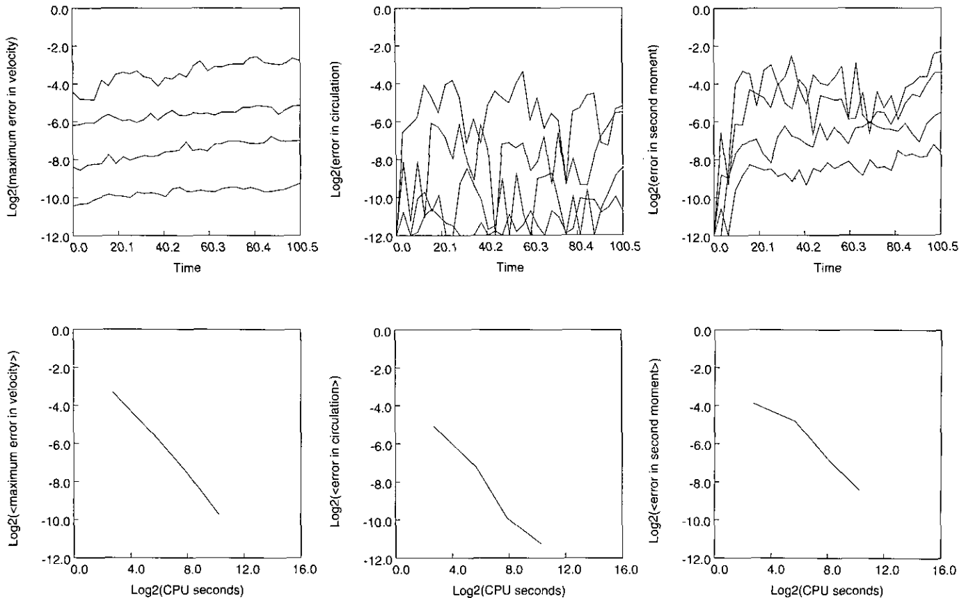
FIG. 20. Errors for Perlman's test case, with an adaptive grid reconnected at every step. First row: Relative L^\infty error in velocity, circulation errors, and second moment errors versus time. Second row: Time-averaged quantities versus Cray-2 CPU time. The four runs plotted used the following parameters: mesh tolerances \epsilon = 0.064, 0.016, 0.004, and 0.001 ; N = 50, 205, 725, and 2709 vertices; n = 64, 96, 128, and 192 time steps.
