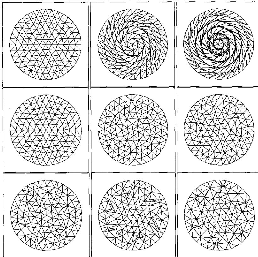
FIG. 16. Fixed (top row) and Delaunay (second row) triangulations at times t = 0, 2\pi, and 4\pi (left to right), and Delaunay triangulations at later times t = 8\pi, 16\pi, and 32\pi (last row).
