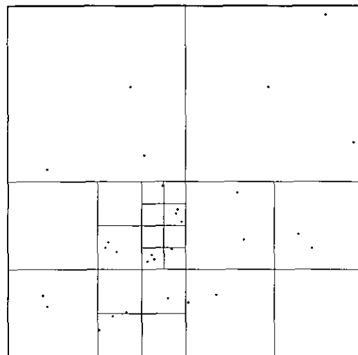
FIG. 9. Adaptive cell structure with no more than three points per cell.
