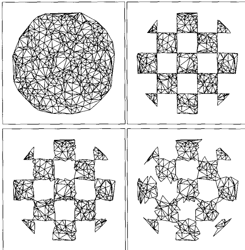
FIG. 12. The original and (alternate cells of the) subdivided triangulation with N = 500 and q = 0.02, 0.08, and 0.32 . The subdivided triangulations have 1146, 750, and 507 vertices, respectively.
