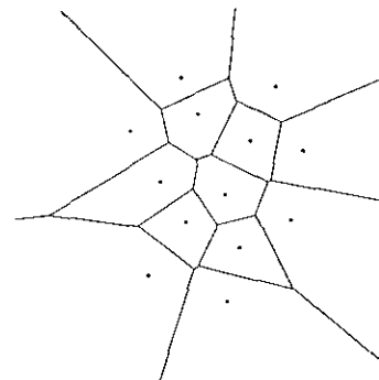
FIG. 4. Voronoi diagram associated with a set of points.
