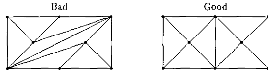
FIG. 3. Good and bad triangulations of a simple point set Z .
