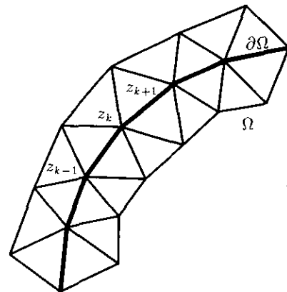
FIG. 28. Symmetric extension of the triangulation beyond \partial\omega .
