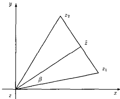
FIG. 2. Triangle \tau_3 .
