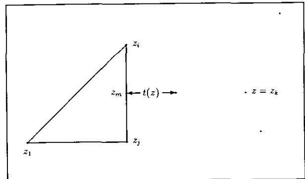
FIG. 6. Geometry of McLain's method.
