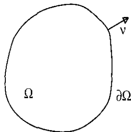
FIG. 27. A domain \Omega and its boundary \partial\Omega .
